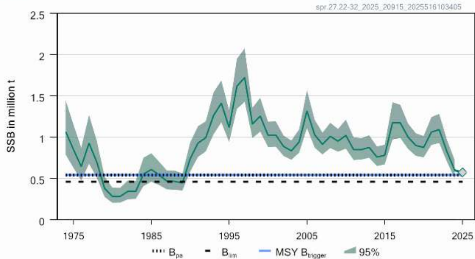
Figure 18 - Sprat in ICES subdivisions 22-32 (Baltic Sea) spawning-stock size above MSY B_{trigger} , B_{pa} , and B_{lim} . (ICES 2025)
