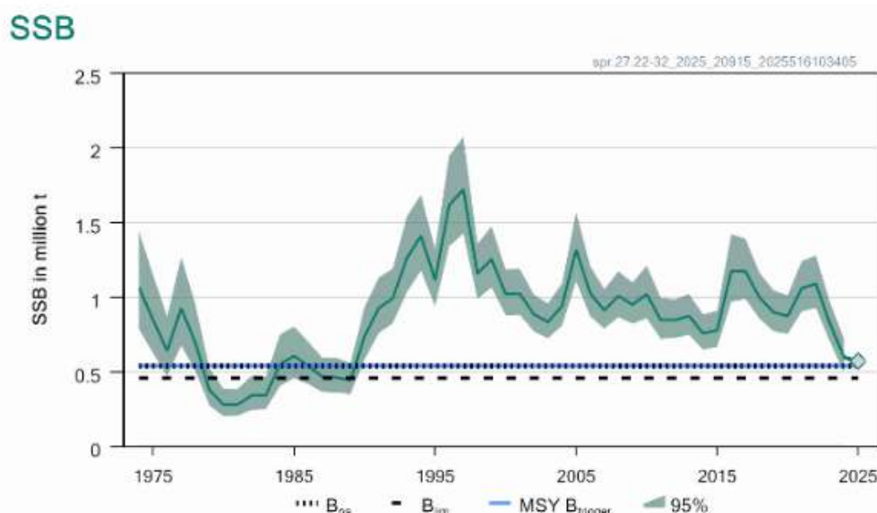
Figure 15 - Sprat in ICES subdivisions 22-32 (Baltic Sea) spawning-stock size above MSY B_{trigger} , B_{PA} , and B_{lim} (ICES 2025)
