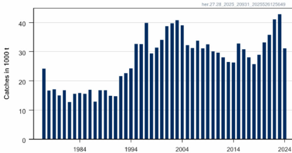
Figure 10. Gulf of Riga herring catches in the Gulf of Riga (ICES subdivision 28.1) 1977-2024 (ICES 2025).
