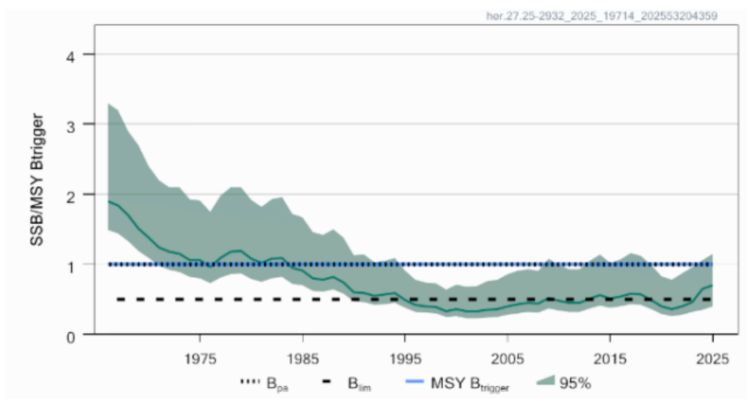
Figure 8. Central Baltic herring, relative spawning biomass and current reference points (ICES)
