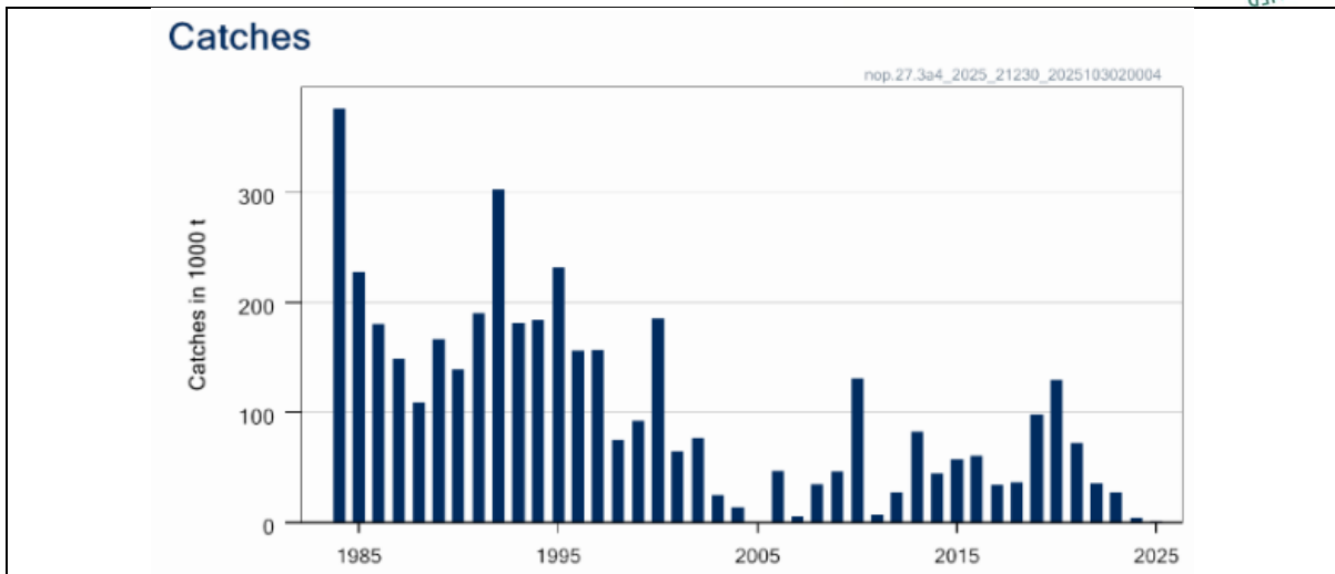
Norway pout catches in Subarea 4 and Division 3.a from 1984 to 2024. Catches in 2024 (shaded in a lighter colour) are up to mid-September. (ICES 2025b).
