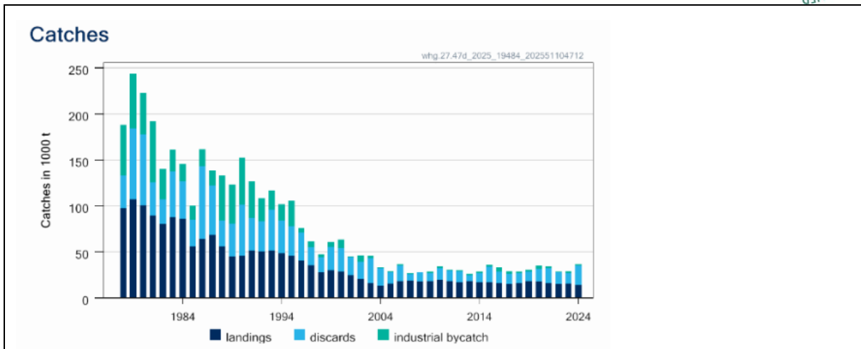
Whiting in Subarea 4 and Division 7.d catches from 1978-2024 (ICES 2025).
