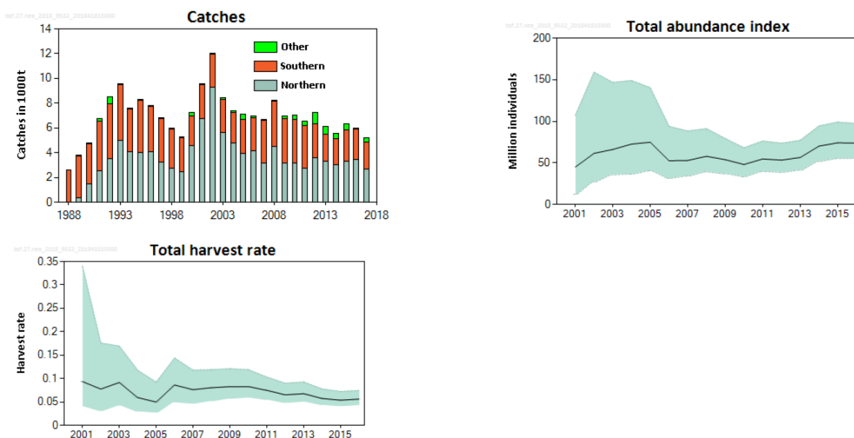
Figure 1. Black scabbardfish in the Northeast Atlantic. Top left: ICES estimates of catches (in thousand tonnes) in the northern part (subareas 6 and 7 and divisions 5.b and 12.b), southern part (Subarea 8 and Division 9.a), and the
