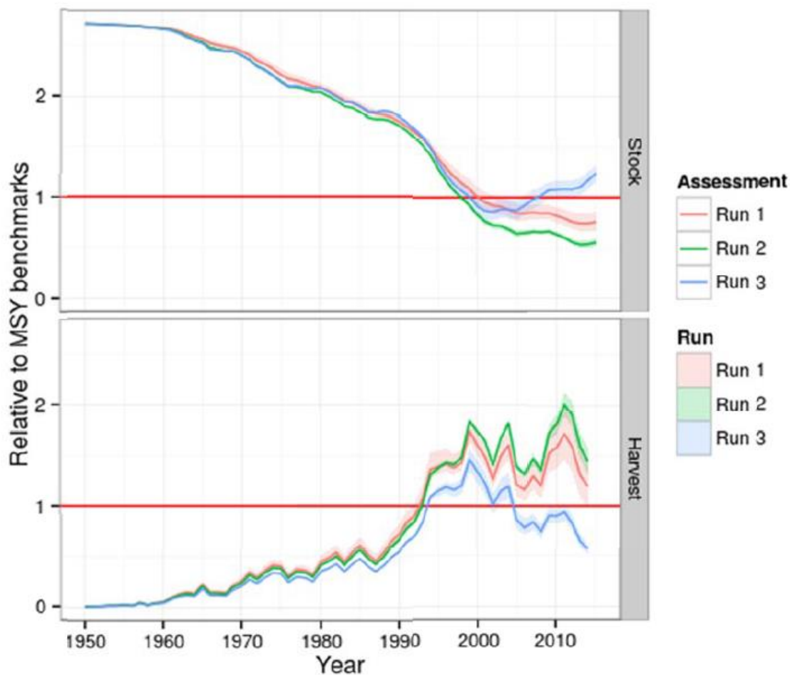
Figure 1. Trajectories of B/B_{MSY} and F/F_{MSY} estimated from the different runs of ASPIC. Lines represent the medians and ribbons the inter-quantiles. Run 1: using USA LL CPUE; Run 2: using Japanese LL CPUE; and Run 3: using Chinese Taipei LL CPUE.
