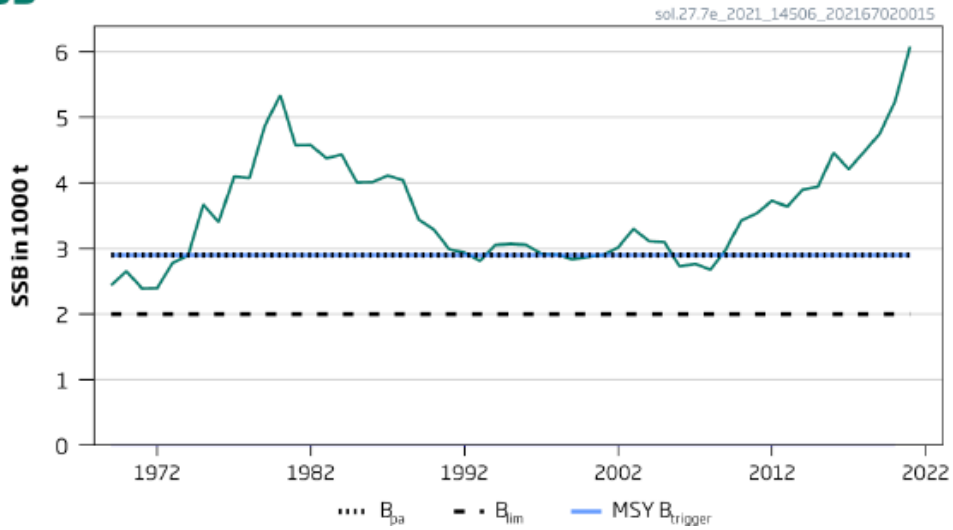
Figure 2. Sole in ICES in Division 7.e. Summary of the stock assessment. Spawning stock biomass. ICES 2021
