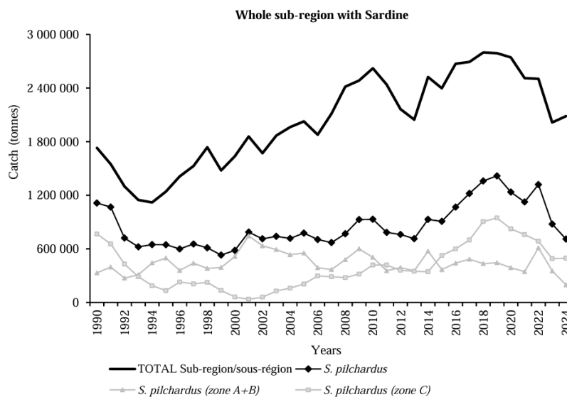
Figure 1. Total catch of small pelagic species and sardine catch in the whole subregion from 1990 to 2024 (FAO 2025).
