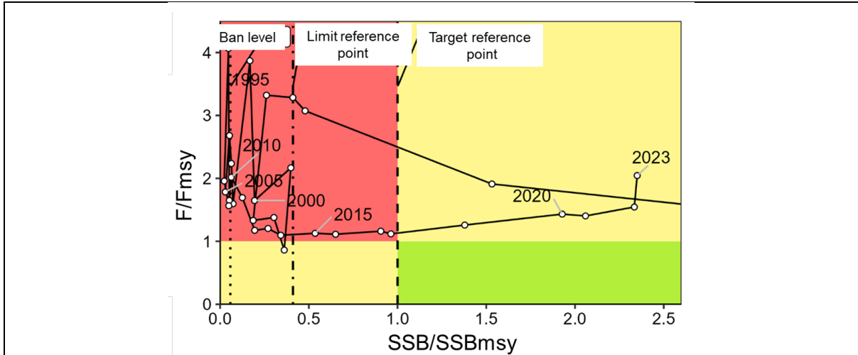
Figure 2. Kobe plot indicating historical and current status of Japanese sardine in relation to MSY-based reference points (NPFC 2024)
