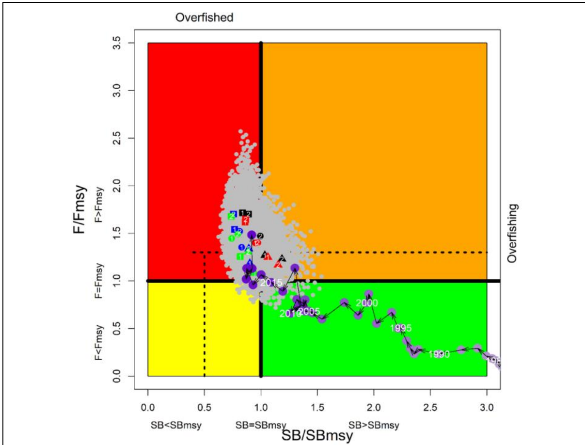
Aggregated Indian Ocean stock assessment Kobe plot for bigeye tuna. Coloured points represent stock status estimates from each of the 24 models. Purple dots represent the time series of stock status estimates. Grey dots represent uncertainty from individual models. Dashed lines indicate IO bigeye tuna limit reference points (IOTC 2023).
