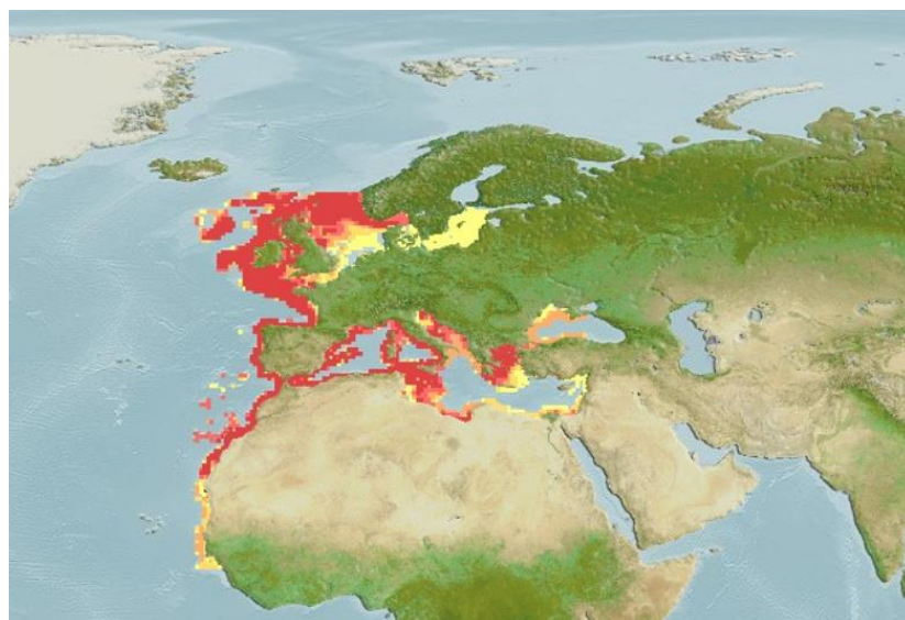
Figure 1. Distribution maps for Capros aper (Boarfish), with modelled year 2050 native range map based on IPCC RCP8.5 emissions scenario. www.aquamaps.org , version 10/2019.
