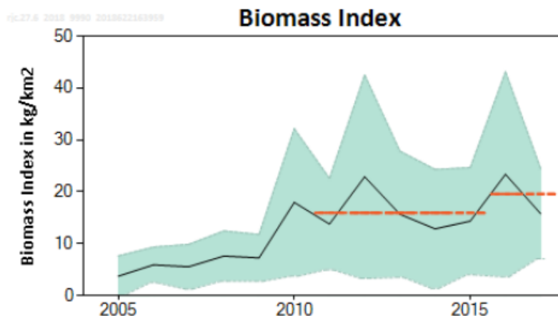
Figure 2. Mean biomass (kg km -2 [IGFS-WIBTS-Q4]) and the 95% CI area. Dashed lines show the mean stock size indicator values for 2011–2015 and 2016–2017. (Source: ICES 2018)
