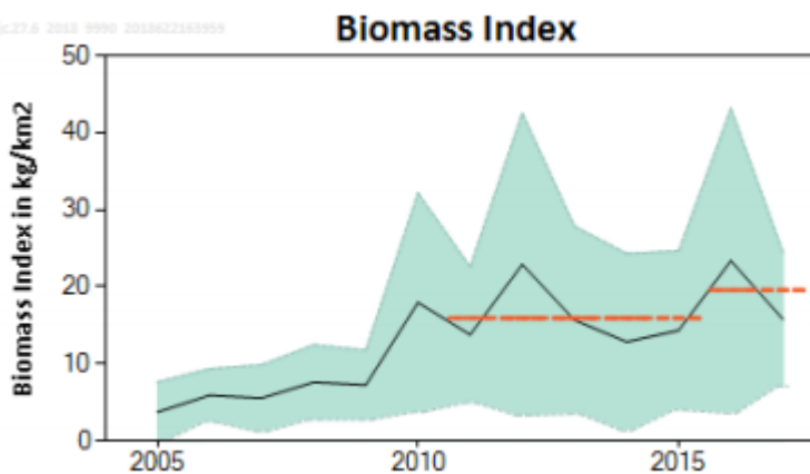
Figure 2. Thornback ray in Subarea 6. Mean biomass (kg km -2 [IGFS-WIBTS-Q4]) and the 95% CI area. Dashed lines show the mean stock size indicator values for 2011–2015 and 2016–2017. (Source: ICES, 2018)
