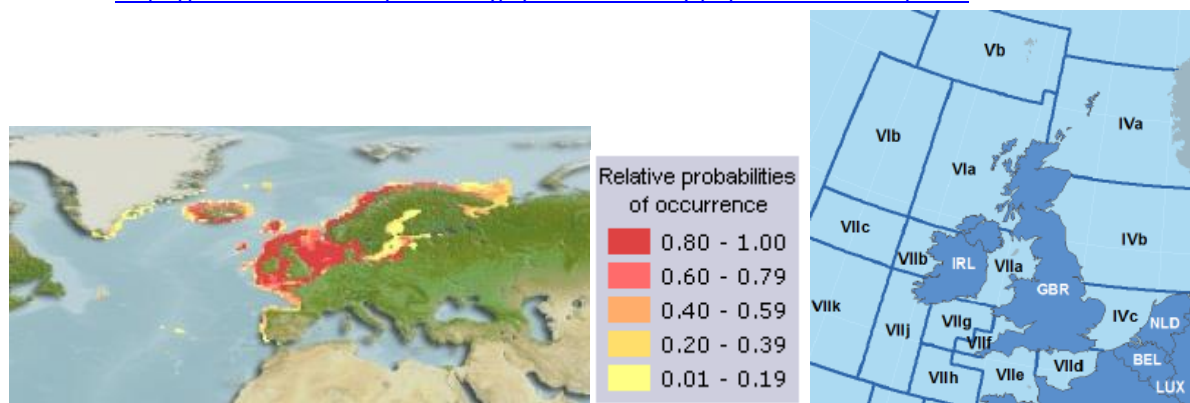
*Figure 1. Left: Distribution of European plaice Pleuronectes platessa
