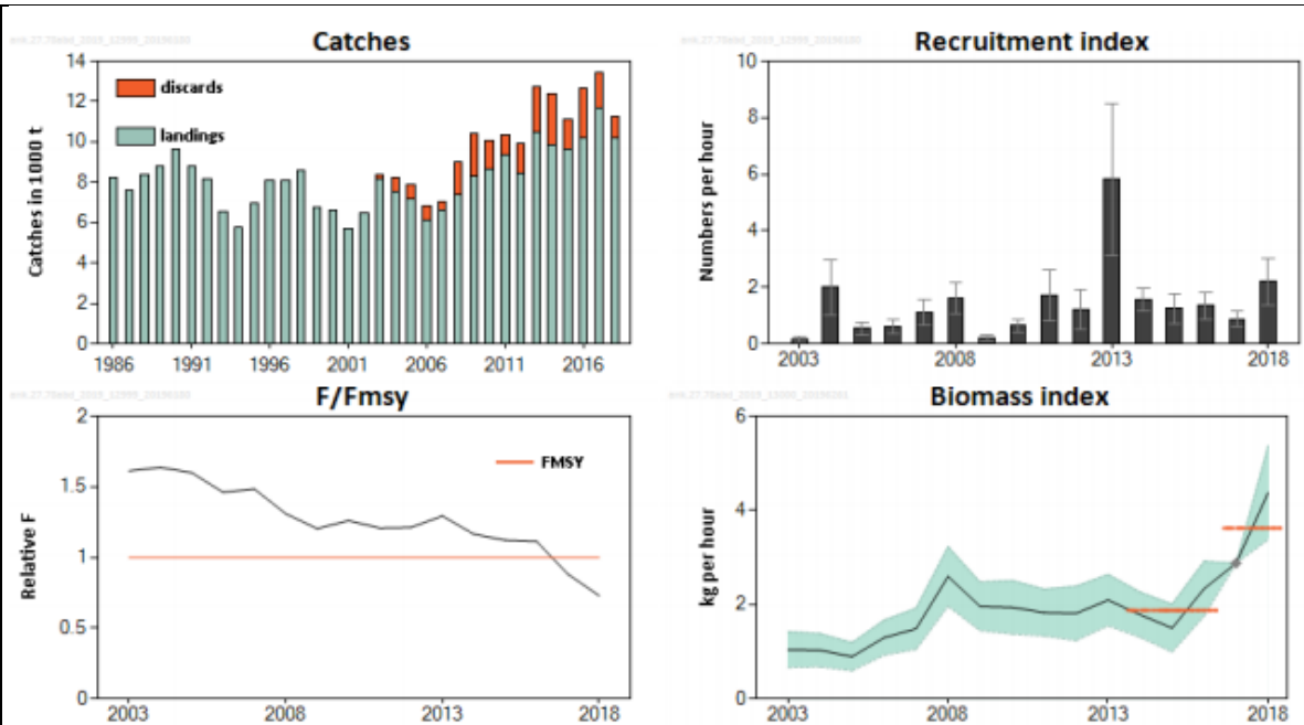
Figure 2. L. budegassa in divisions 7.b-k, 8.a–b, and 8.d. Summary of the stock assessment. The biomass and recruitment indices from the combined surveys are displayed with confidence intervals (95%). The 2017 point in the biomass index is imputed, and its confidence interval is not provided owing to the differing method. The short orange horizontal lines represent the mean biomass index in the most recent 2 years and the preceding 3 years (source: ICES, 2019).
