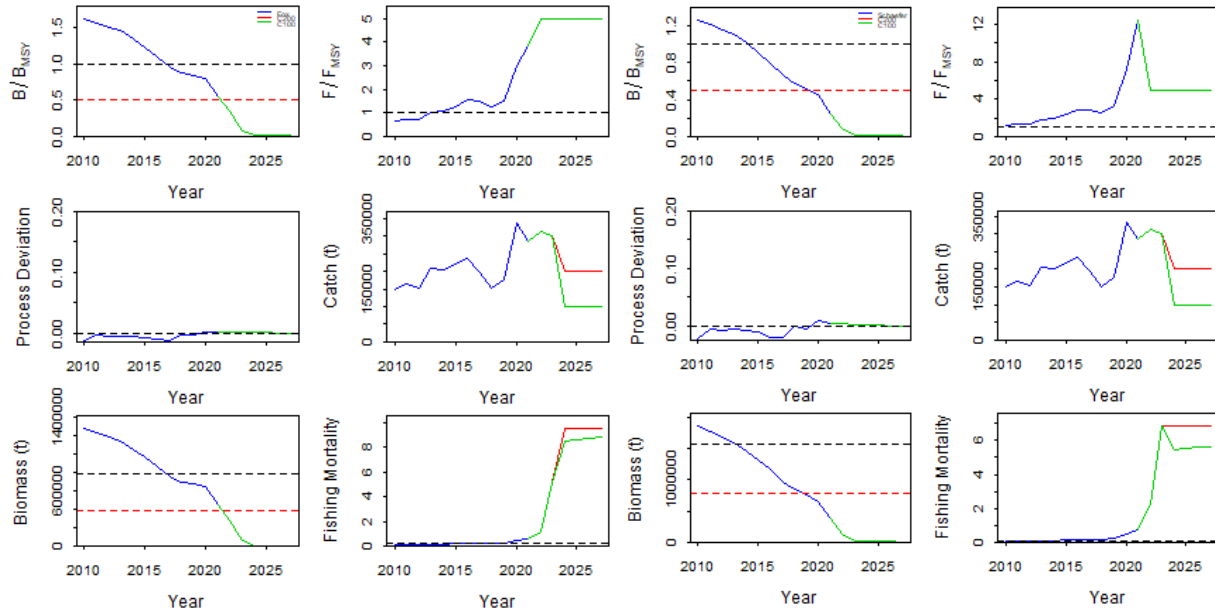
Figure 16. Simulation of biomass and catch trajectory on the basis of setting a TAC according to the catch (average of 10 years) for flat sardinella . For projections based on Fmsy, the situation is also worrying for both models (Figure 17).
