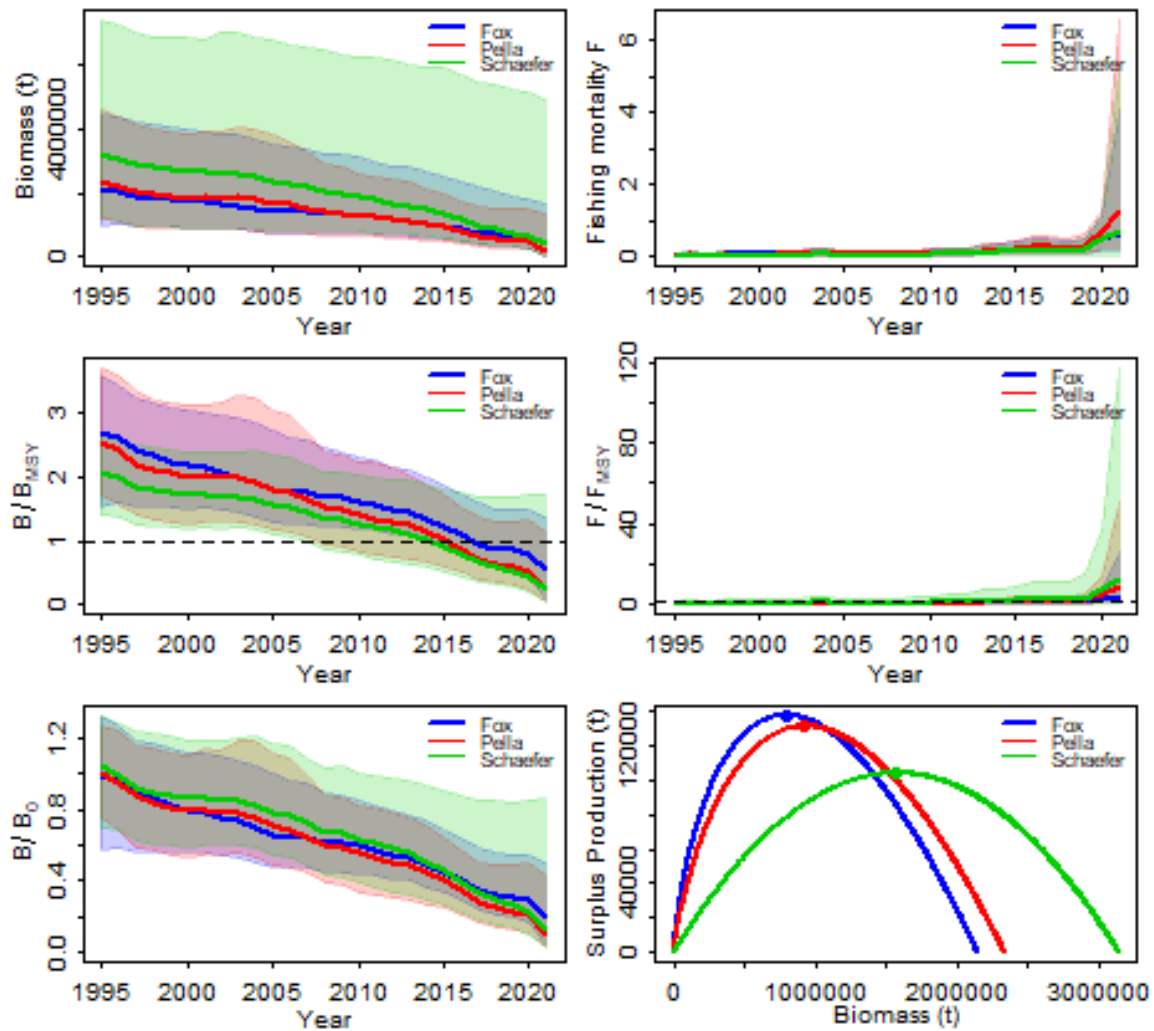
Figure 9 : Analysis performed on the different models applied to flat sardinella and predicting the trends in biomass and fishing mortality (upper panels), biomass relative to BMSY ( B/B_{MSY} ) and fishing mortality relative to FMSY ( F/F_{MSY} ) (middle panels) and biomass relative to K ( B/K ) and surplus production curve (bottom panels) for each scenario from the model
