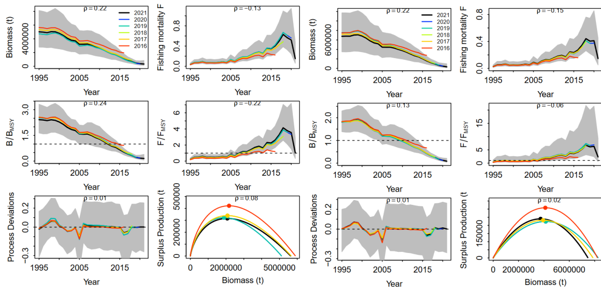
Figure 7 : Retrospective analysis performed on the Schaefer (left) and Fox (right) models, by removing one year at a time sequentially ( n=5 ) and predicting the trends in biomass and fishing mortality (upper panels), biomass relative to B_{MSY} ( B/B_{MSY} ) and fishing mortality relative to F_{MSY} ( F/F_{MSY} ) (middle panels) and biomass relative to K ( B/K ) and surplus production curve (bottom panels) for each scenario from the model fits to the round sardinella.
