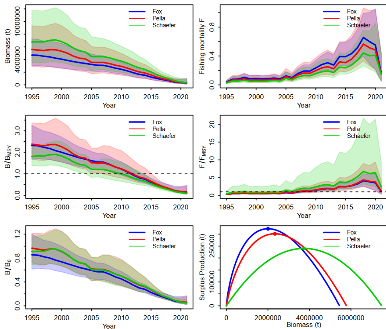
415 416 Figure 6 : Analysis performed on the different models applied to round sardinella and predicting the 417 trends in biomass and fishing mortality (upper panels), biomass relative to BMSY ( B/B_{MSY} ) and fishing 418 mortality relative to FMSY ( F/F_{MSY} ) (middle panels) and biomass relative to K ( B/K ) and surplus 419 production curve (bottom panels) for each scenario from the model.
