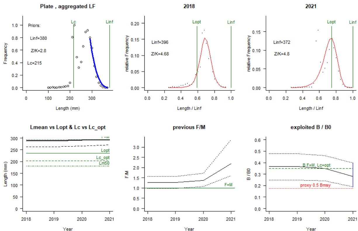
Figure 13 : Top-left: aggregated length frequency (LF) data and priors for L_c , L_{inf} , and Z/k . Top-mid and top-right: dots are the length-frequency data for the first and last years, and the red line is the fit of the data to the LBB master equation, for 2018 and 2021 respectively. Bottom-left: mean length ( L_{mean} , bold black curve) relative to L_{opt} , and L_c (dashed black curve) relative to L_{c_{opt}} . Bottom mid: relative fishing mortality F/M (black curve), with approximate 95% confidence limits (dotted lines), and reference level ( F = M , green horizontal line). Bottom right: relative biomass B/B_0 (black curve) with approximate 95% confidence limits (dotted black curves), and a proxy for BMSY (green dashed line), and a proxy for Bpa or 0.5 BMSY (red dotted line).
