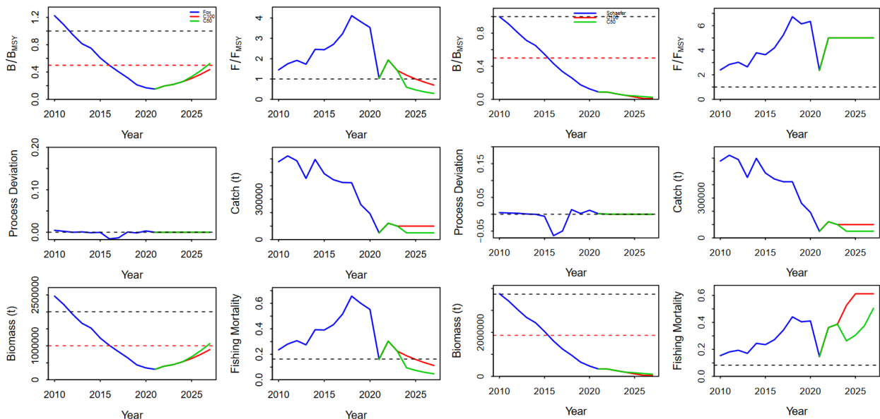
Figure 14. Simulation of biomass and catch trajectory on the basis of setting a TAC according to the catch of the last year and the average of 3 years for round sardinella .
