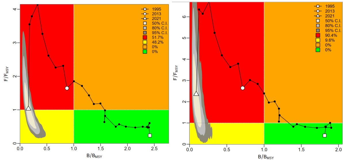
Figure 8 - JABBA surplus production phase plot for the Schaefer model (left) and Fox model (right) for round sardinella showing trajectories of the catches in relation to BMSY and MSY (top panel) and Kobe phase plot showing estimated trajectories (1995-2021) of B/BMSY and F/FMSY for the Bayesian state-space surplus production model for the round sardinella (bottom panel). Different grey shaded areas denote the 50%, 80%, and 95% credibility interval for the terminal assessment year. The probability of terminal year points falling within each quadrant is indicated in the figure legend.
