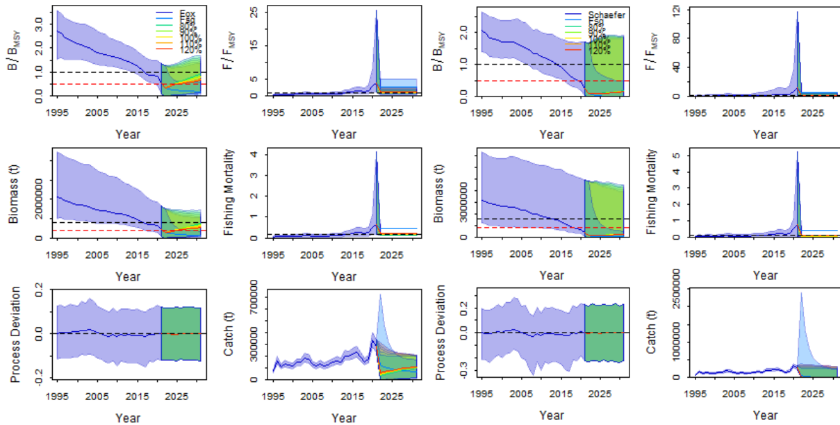
Figure 17. Simulation of biomass and fishing mortality trajectories based on the Fmsy projection for flat sardinella
