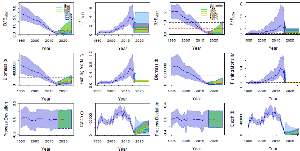
Figure 15. Simulation of biomass and fishing mortality trajectories based on the Fmsy projection for round sardinella.
