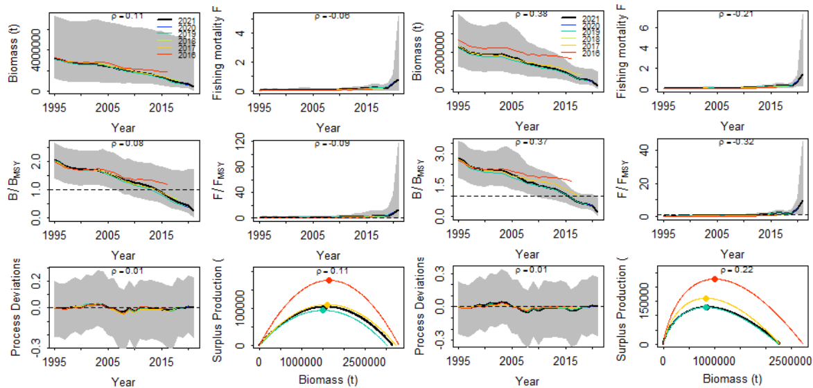
Figure 10 : Retrospective analysis performed on the Schaefer (left) and Fox (right) models, by removing one year at a time sequentially ( n=5 ) and predicting the trends in biomass and fishing mortality (upper panels), biomass relative to BMSY ( B/B_{MSY} ) and fishing mortality relative to FMSY ( F/F_{MSY} ) (middle panels) and biomass relative to K ( B/K ) and surplus production curve (bottom panels) for each scenario from the model fits to the flat sardinella.
