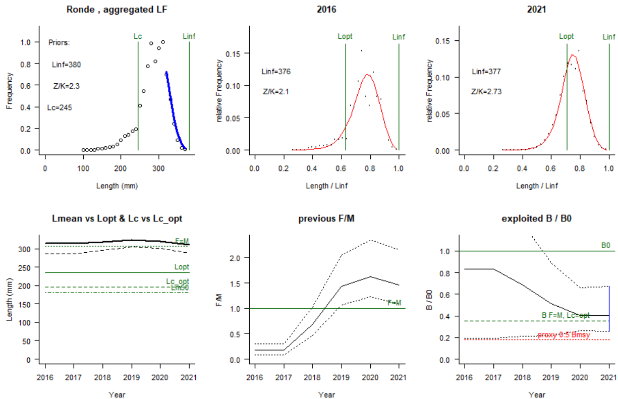
Figure 12: Results of the LBB for round sardinella. Top-left: aggregated length frequency (LF) data and priors for L_c , L_{inf} , and Z/k . Top-mid and top-right: dots are the length-frequency data for the first and last years, and the red line is the fit of the data to the LBB master equation, for 2016 and 2021 respectively. Bottom-left: mean length ( L_{mean} , bold black curve) relative to L_{opt} , and L_c (dashed black curve) relative to L_{c_{opt}} . Bottom mid: relative fishing mortality F/M (black curve), with approximate 95% confidence
