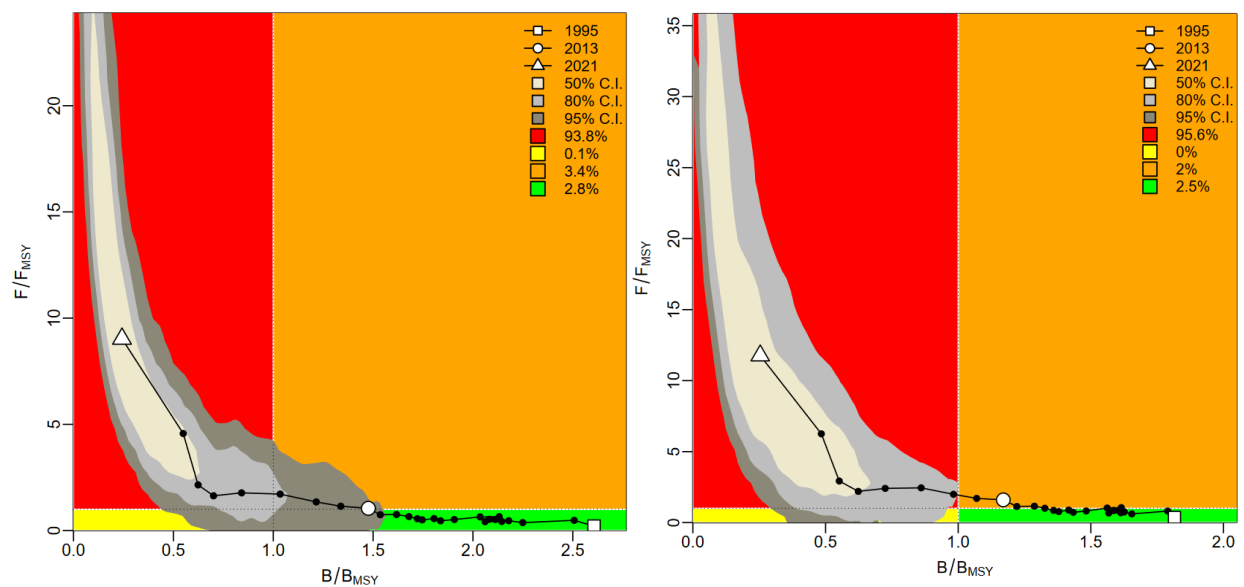
Figure 11 - JABBA surplus production phase plot for the Fox model (right) and Schaefer model (left) for flat sardinella showing trajectories of the catches in relation to BMSY and MSY (top panel) and
